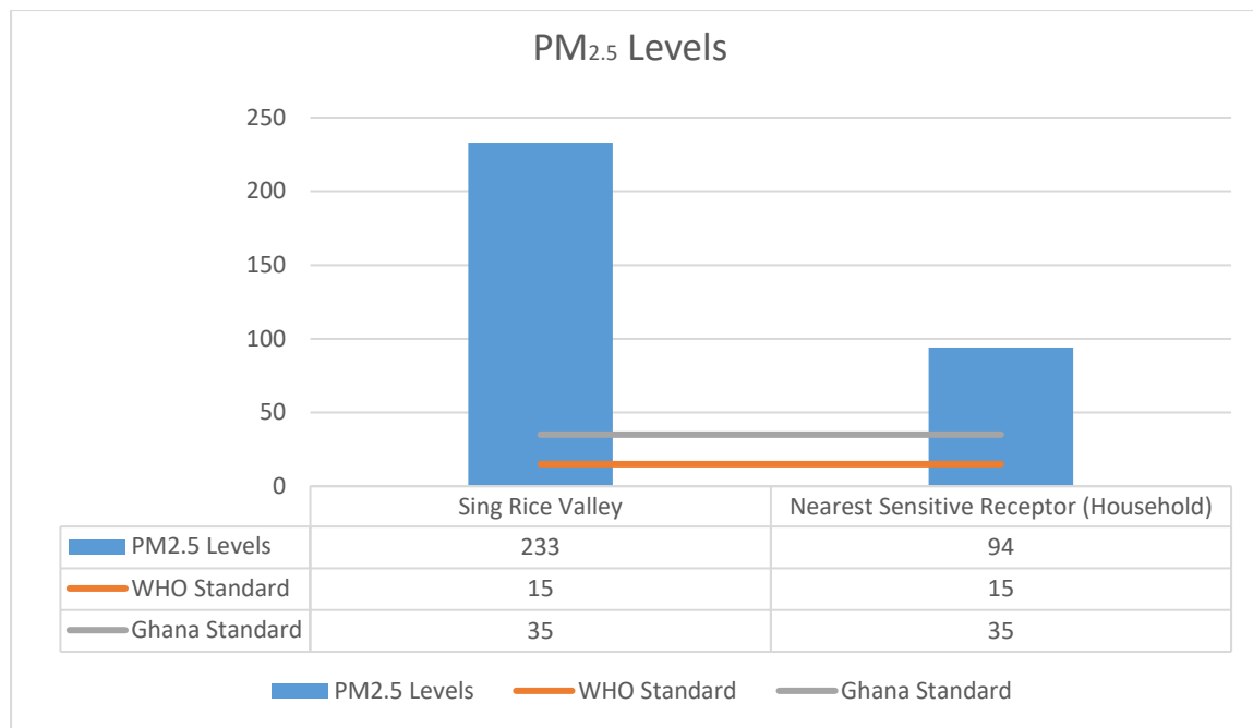
Figure 5-19: Graph showing compliance and or exceedance of PM 2.5 particulates to GSA/WHO Standards (SAL Consult, 2025)
