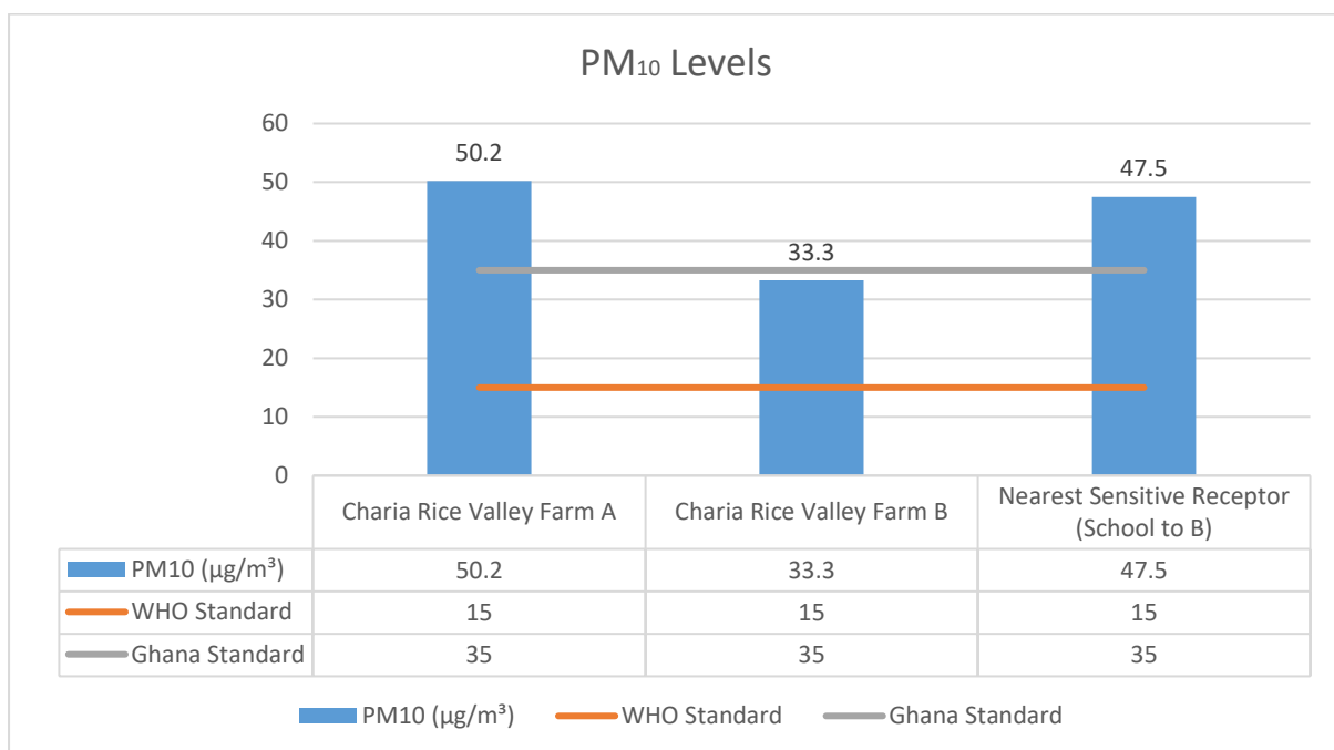
Figure 5-17: Graph showing compliance and or exceedance of PM 10 particulates to GSA/WHO Standards (SAL Consult, 2025)
