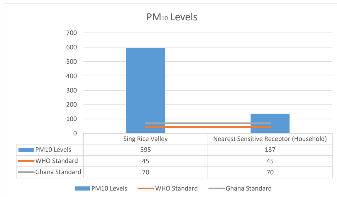
Figure 5-20: Graph showing compliance and or exceedance of PM 10 particulates to GSA/WHO Standards (SAL Consult, 2025)
