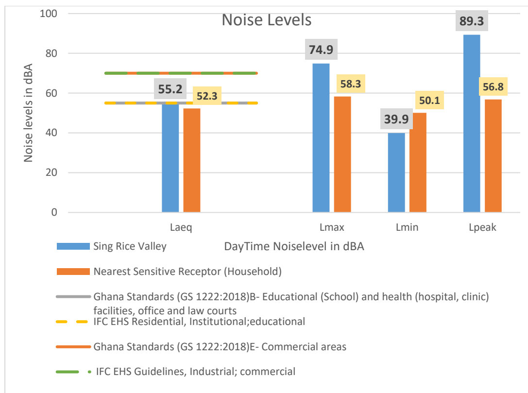
Figure 5-21: Ambient noise levels measured at the Valley and nearest sensitive receptors (SAL Consult, 2025)
