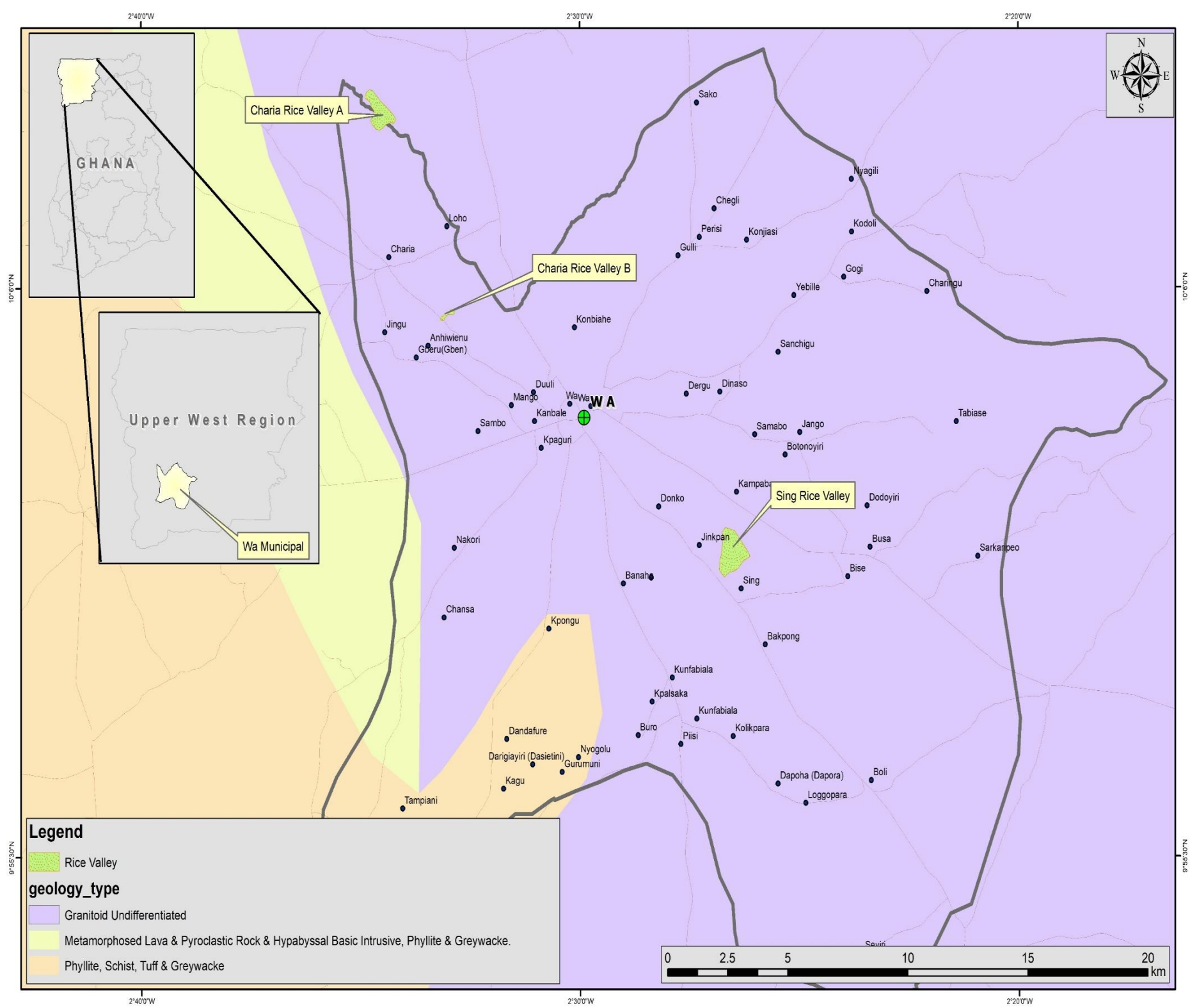
Figure 5-10: Geology Map of the Wa Municipal Area (Source: SAL Consult, 2025)
