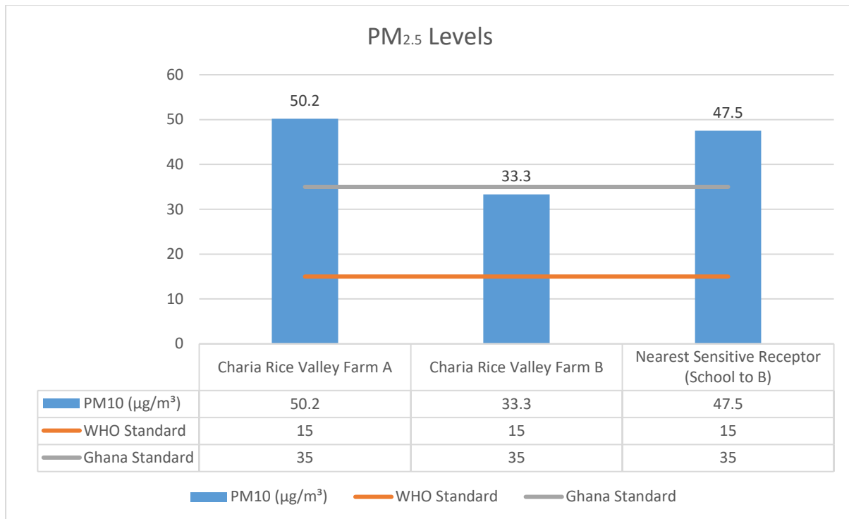
Figure 5-16: Graph showing compliance and or exceedance of PM 2.5 particulates to GSA/WHO Standards (SAL Consult, 2025)
